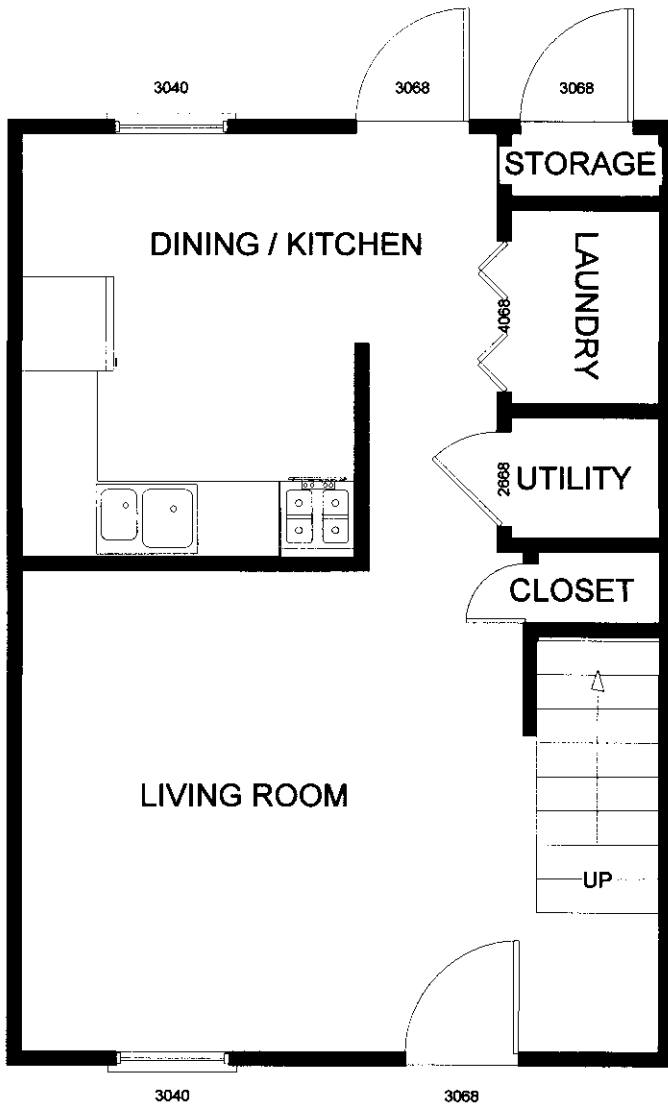
TYPICAL 1st FLOOR - 2 BEDROOM PLAN 438 sq ft
