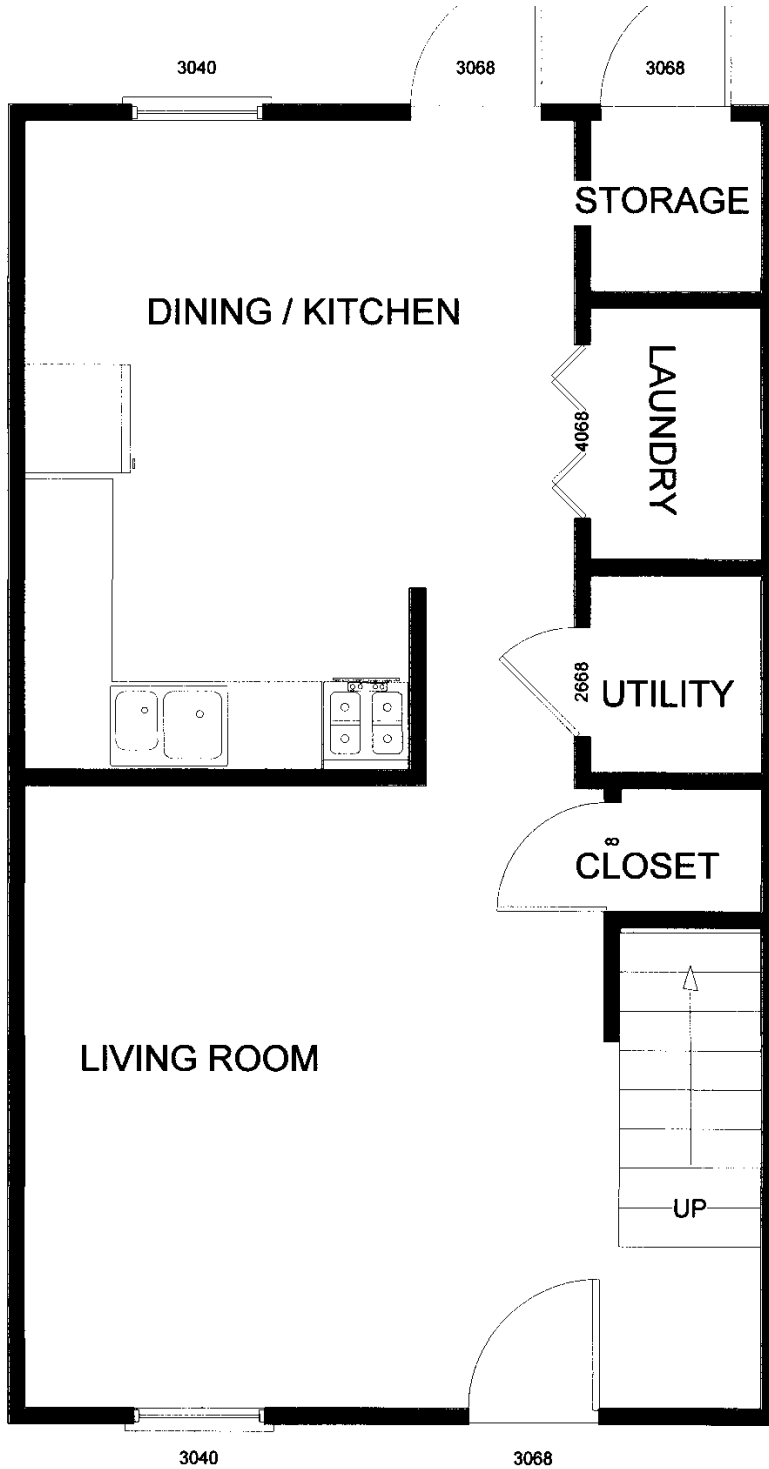
Typical 1st Floor- 3 Bedroom Plan 528 sq ft
