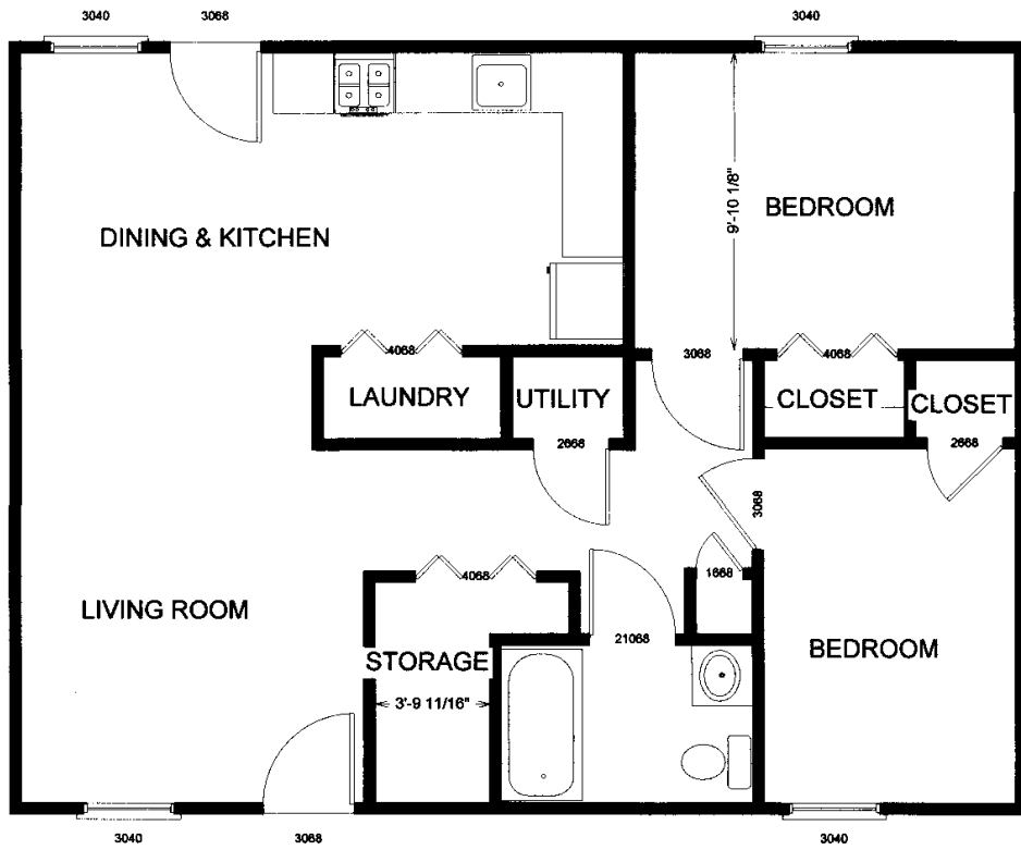
TYPICAL 2 BEDROOM HANDICAP FLOOR PLAN 846 sq ft
