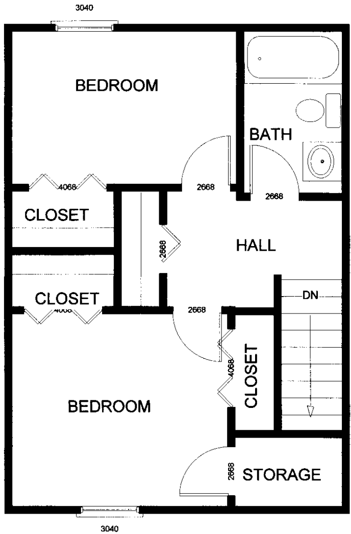
TYPICAL 2nd FLOOR 2 BEDROOM PLAN 437 sq ft
