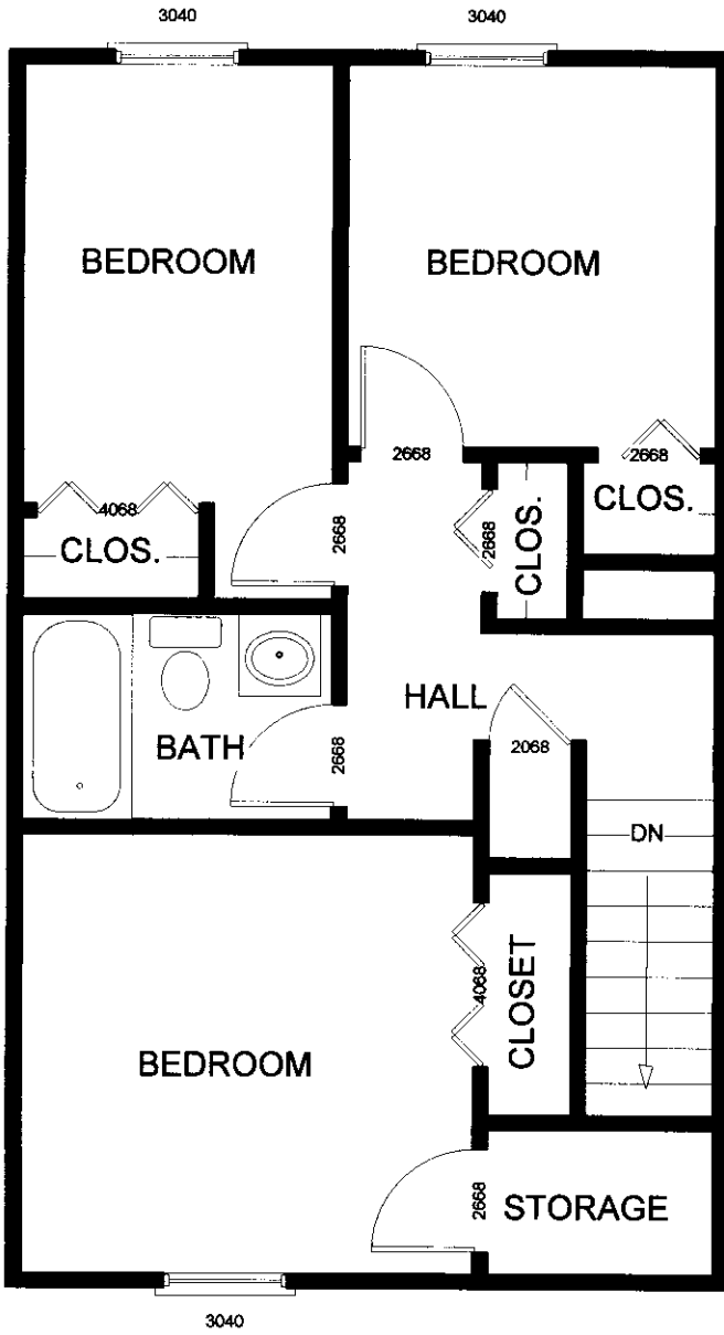
TYPICAL 2nd FLOOR - 3 BEDROOM PLAN 528 sq ft
