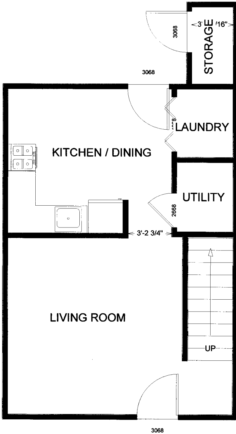
TYPICAL FIRST FLOOR PLAN 436 sq ft
