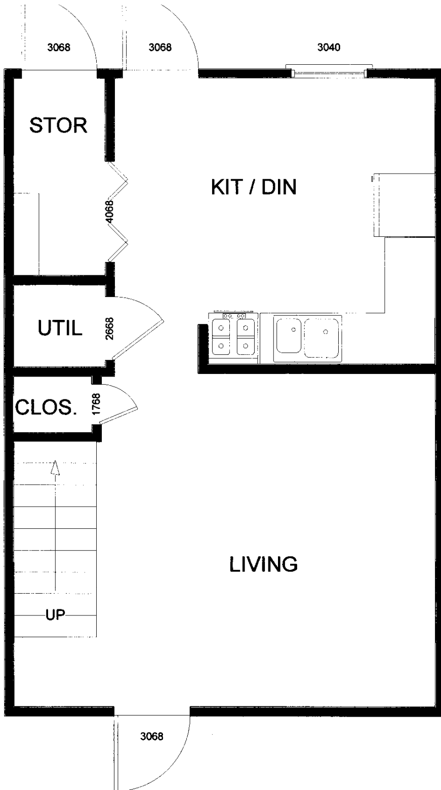
TYPICAL FIRST FLOOR PLAN 440 sq ft
